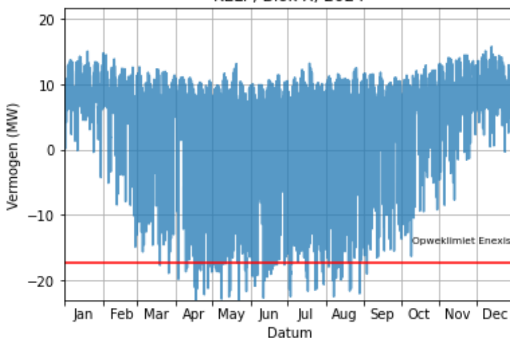
KELP, Blok X, 2024
